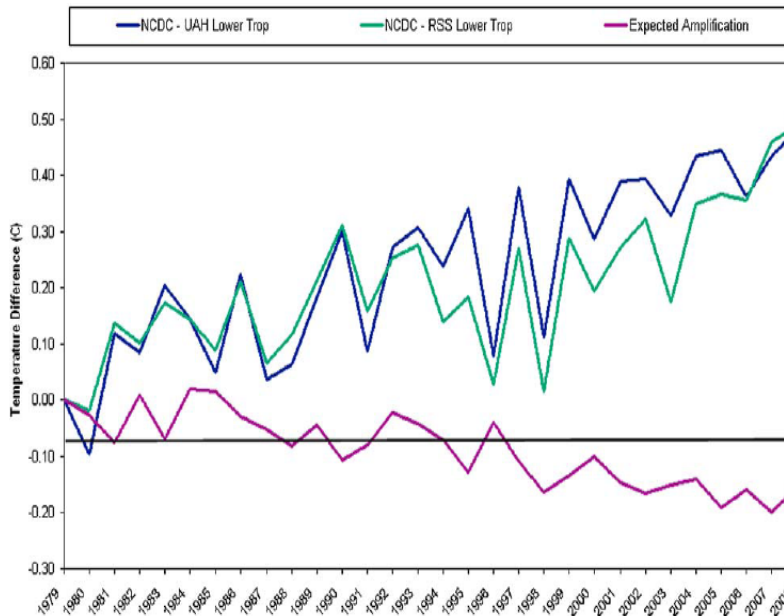
NCDC (terrestrial) minus UAH (satellite: blue) and minus RSS (satellite: green) lower-troposphere annual land temperature differences, 1979-2008. The expected difference (purple) given the model amplification lapse-rate factor of 1.2 is also shown. All differences are zeroed to 1979.
